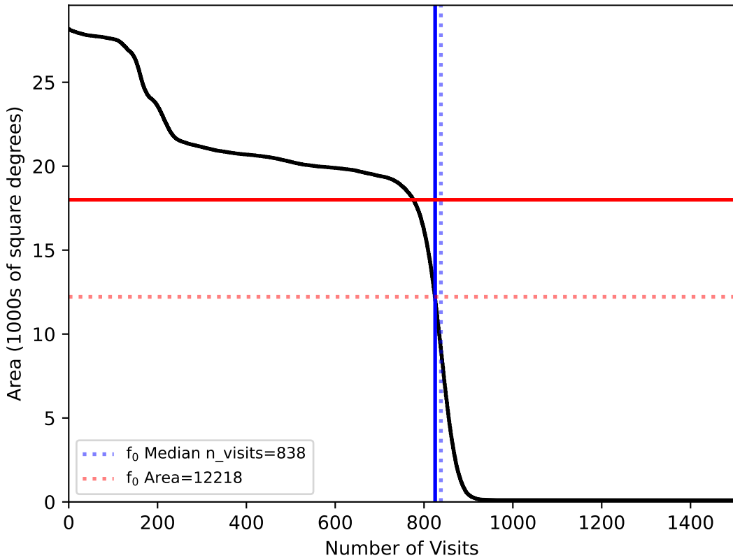
internal_u_expt60_nscale1.5v3.4_10yrs : f0
