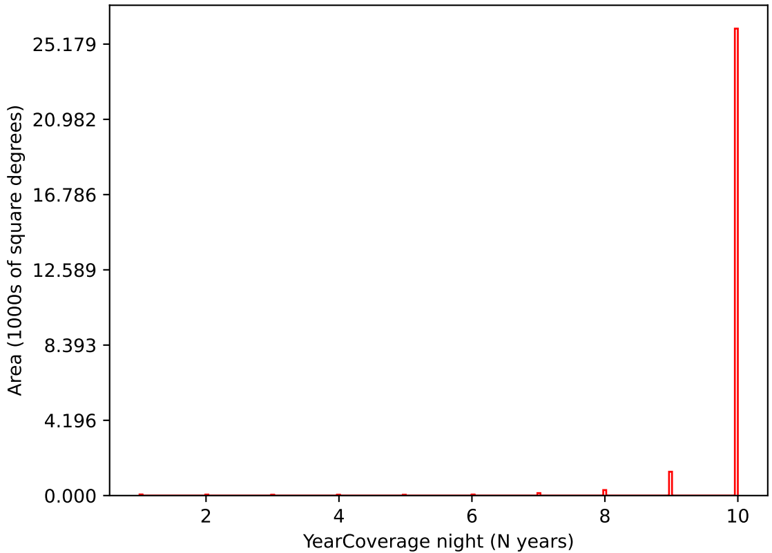
internal_u_expt60_nscale1.5v3.4_10yrs i band: YearCoverage night
