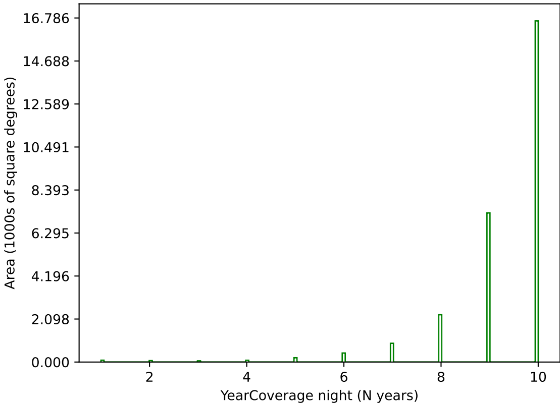
internal_u_expt60_nscale1.5v3.4_10yrs g band: YearCoverage night
