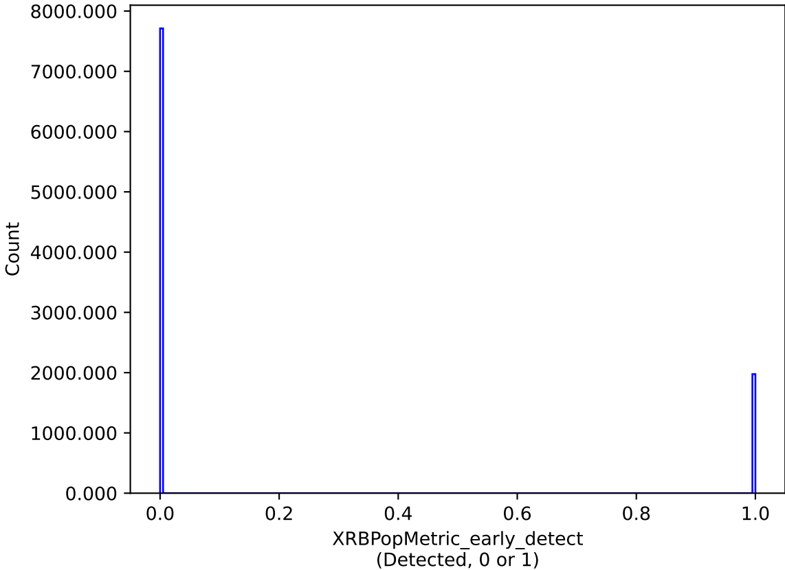
internal_u_expt60_nscale1.5v3.4_10yrs : XRBPoMetric_early_detect
