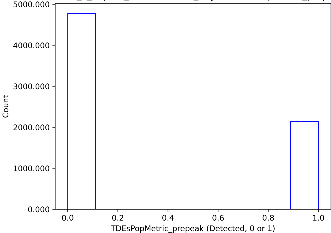
internal_u_expt60_nscale1.5v3.4_10yrs : TDEsPopMetric_prepeak
