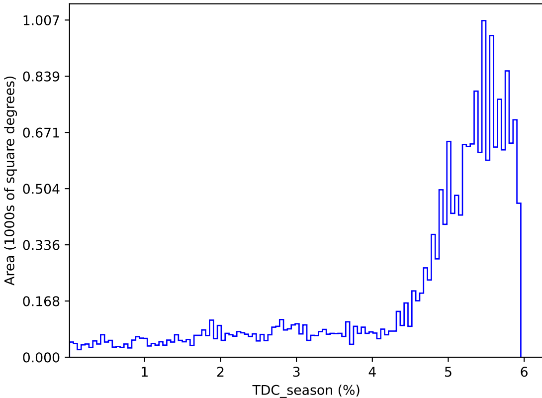
internal_u_expt60_nscale1.5v3.4_10yrs : TDC_season
