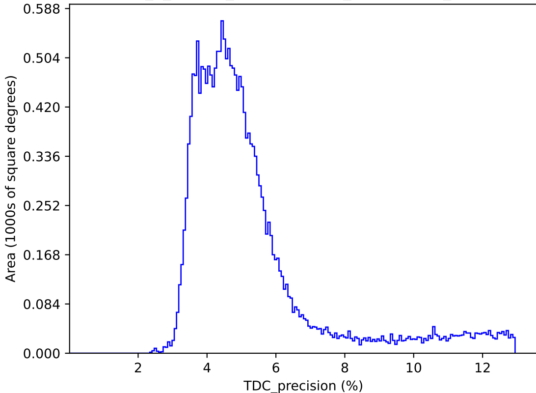
internal_u_expt60_nscale1.5v3.4_10yrs : TDC_precision
