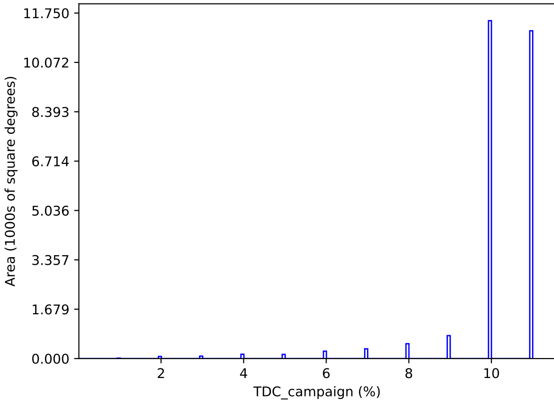
internal_u_expt60_nscale1.5v3.4_10yrs : TDC_campaign
