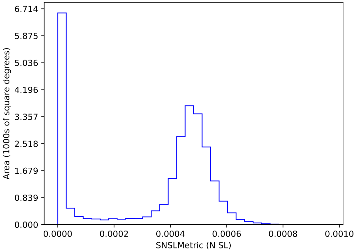
internal_u_expt60_nscale1.5v3.4_10yrs : SNSLMetric
