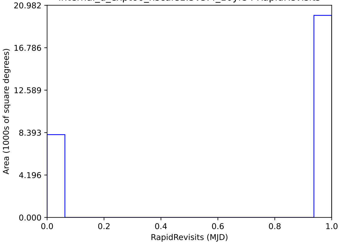
internal_u_expt60_nscale1.5v3.4_10yrs : RapidRevisits
