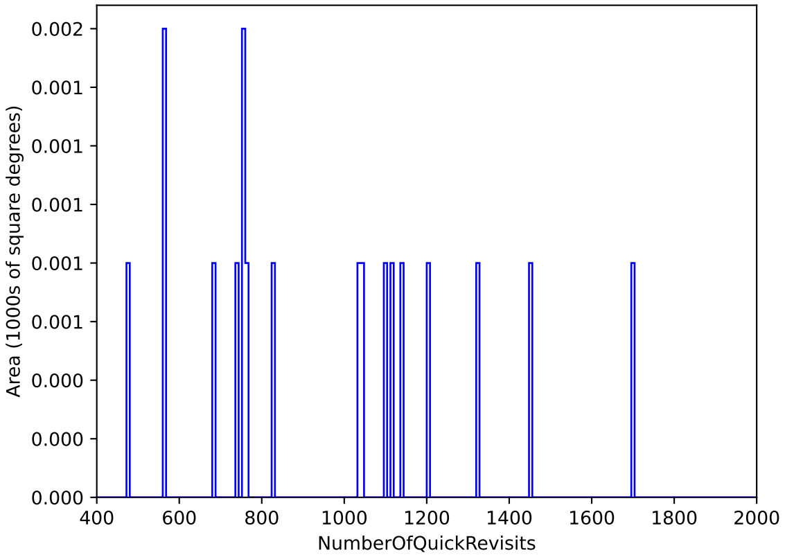
internal_u_expt60_nscale1.5v3.4_10yrs : NumberOfQuickRevisits
