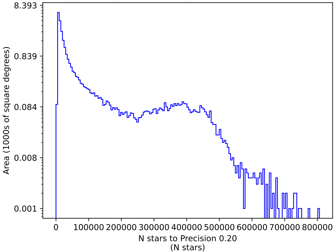
internal_u_expt60_nscale1.5v3.4_10yrs z: N stars to Precision 0.20
