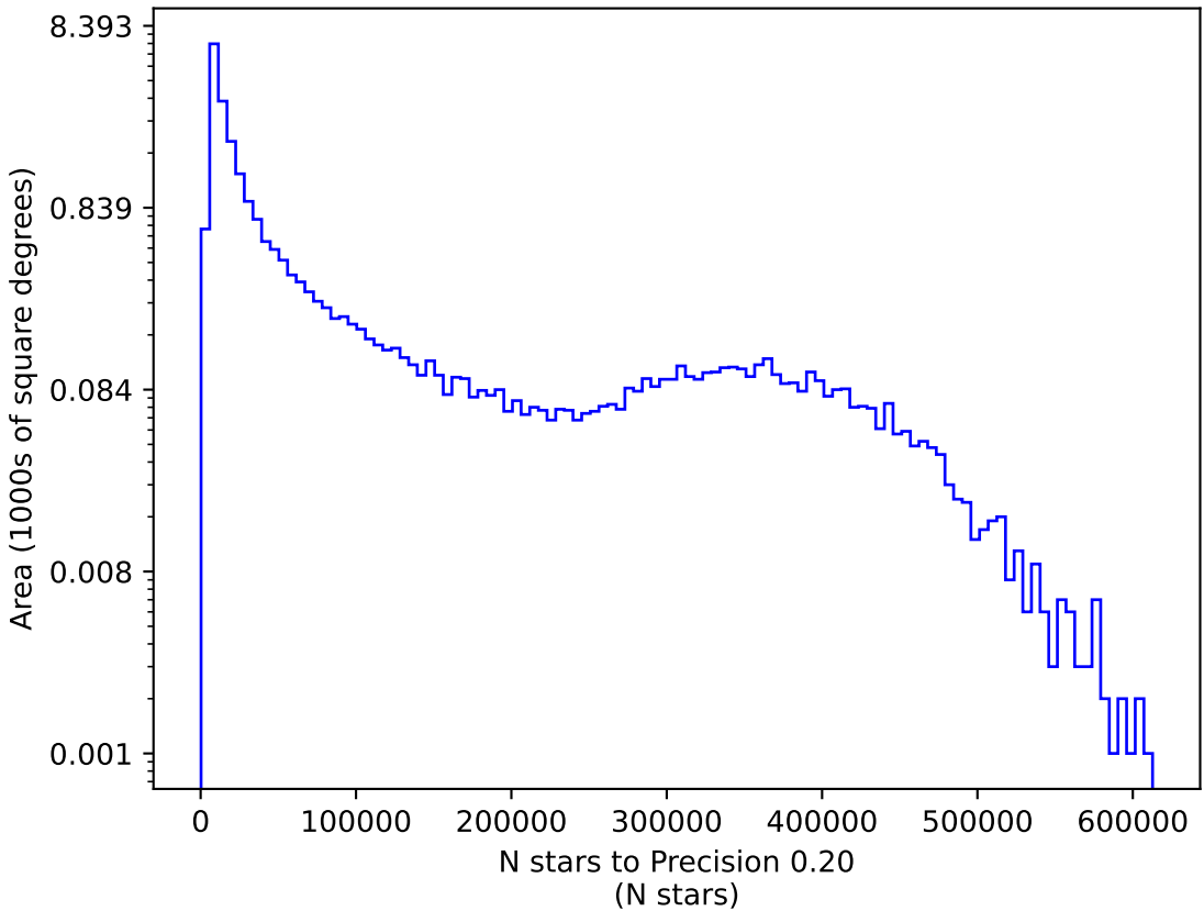
internal_u_expt60_nscale1.5v3.4_10yrs y: N stars to Precision 0.20
