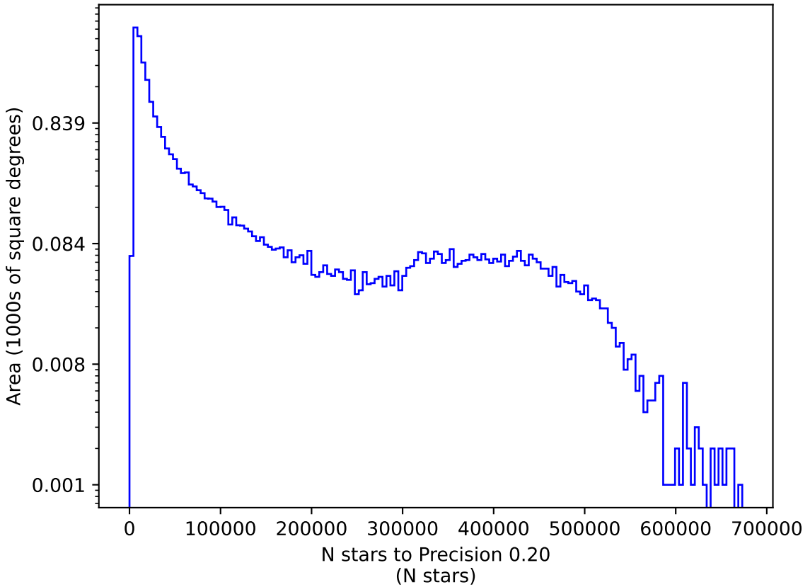
internal_u_expt60_nscale1.5v3.4_10yrs r: N stars to Precision 0.20
