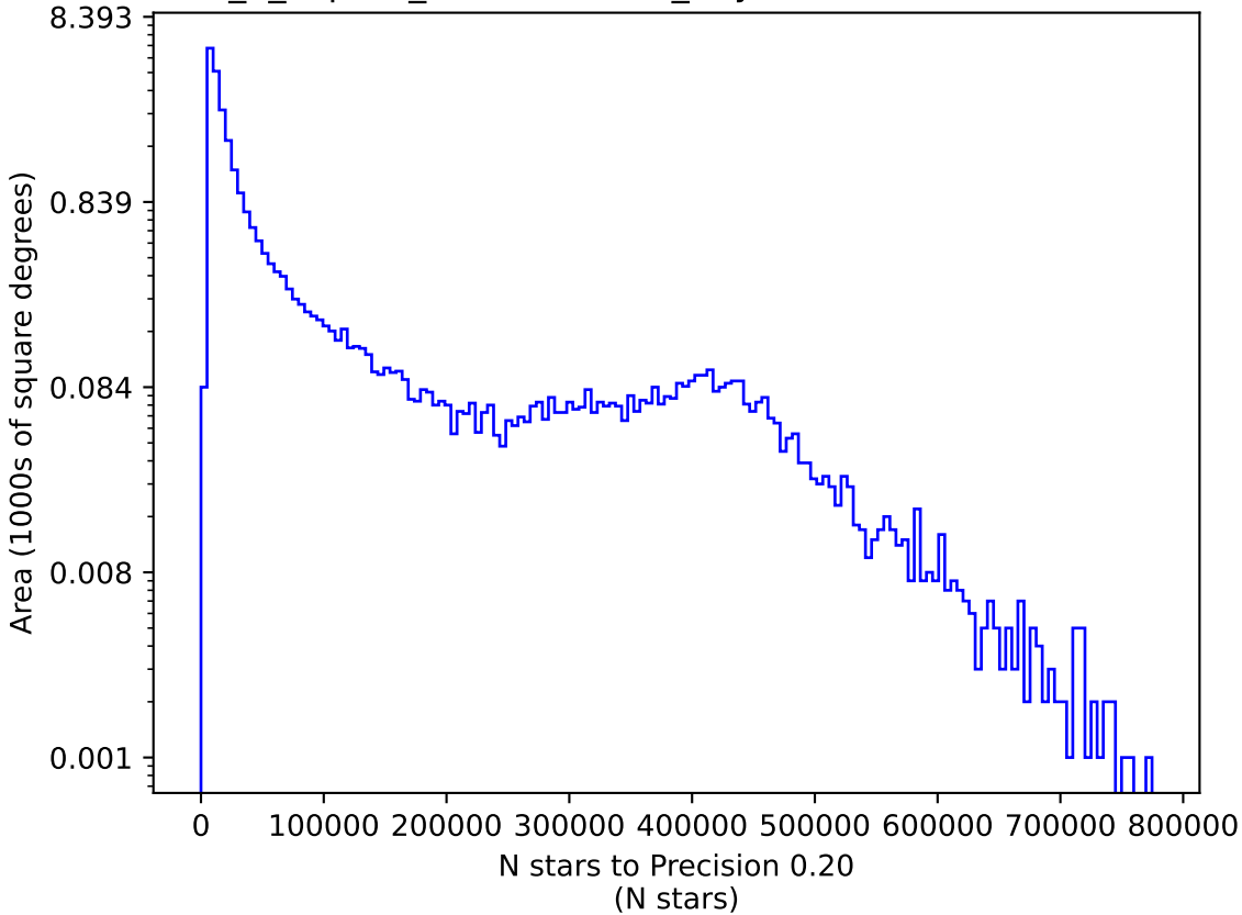
internal_u_expt60_nscale1.5v3.4_10yrs i: N stars to Precision 0.20
