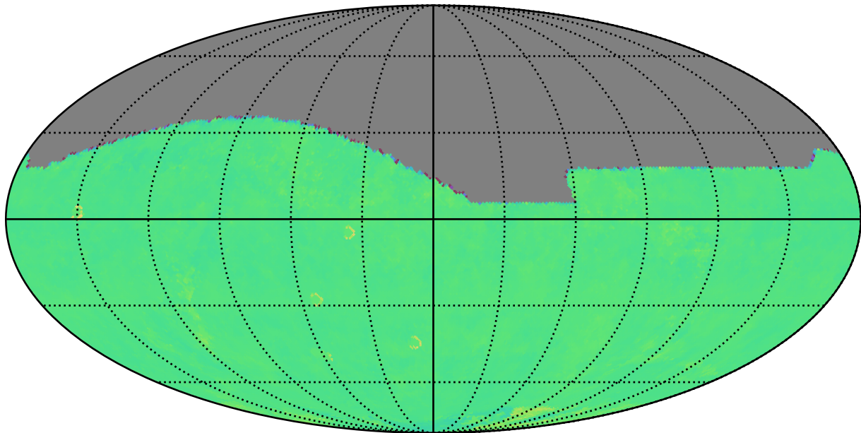
internal_u_expt60_nscale1.5v3.4_10yrs r: Kuiper rotTelPos
