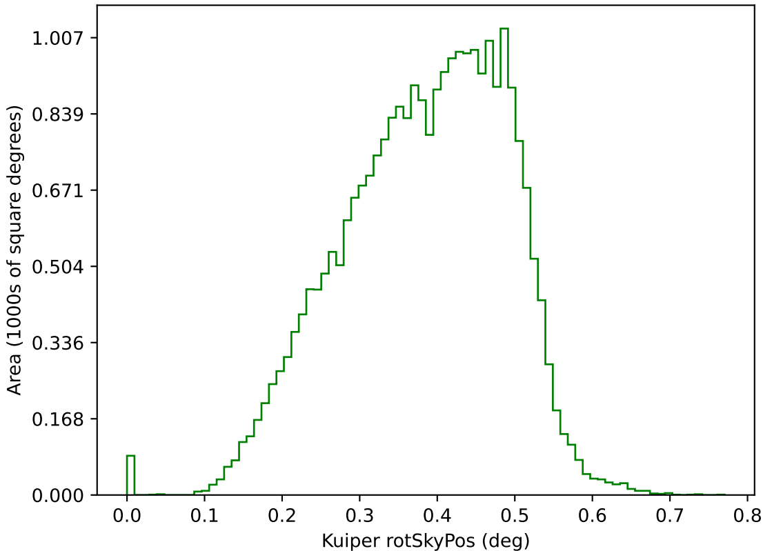
internal_u_expt60_nscale1.5v3.4_10yrs g: Kuiper rotSkyPos
