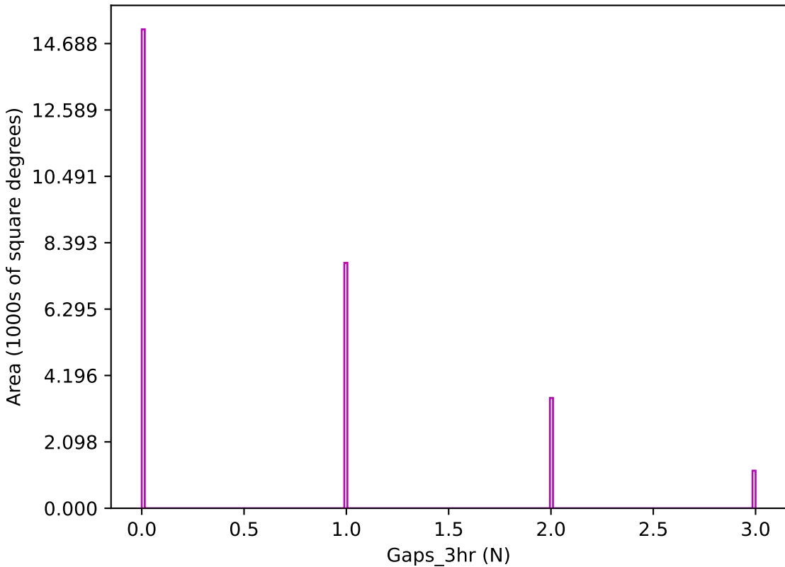
internal_u_expt60_nscale1.5v3.4_10yrs z band: Gaps_3hr
