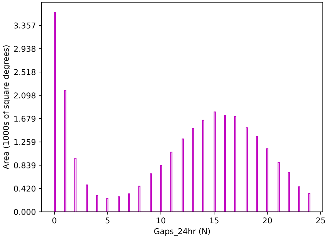
internal_u_expt60_nscale1.5v3.4_10yrs z band: Gaps_24hr
