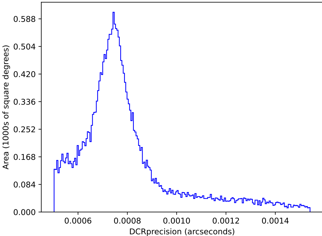
internal_u_expt60_nscale1.5v3.4_10yrs : DCRprecision
