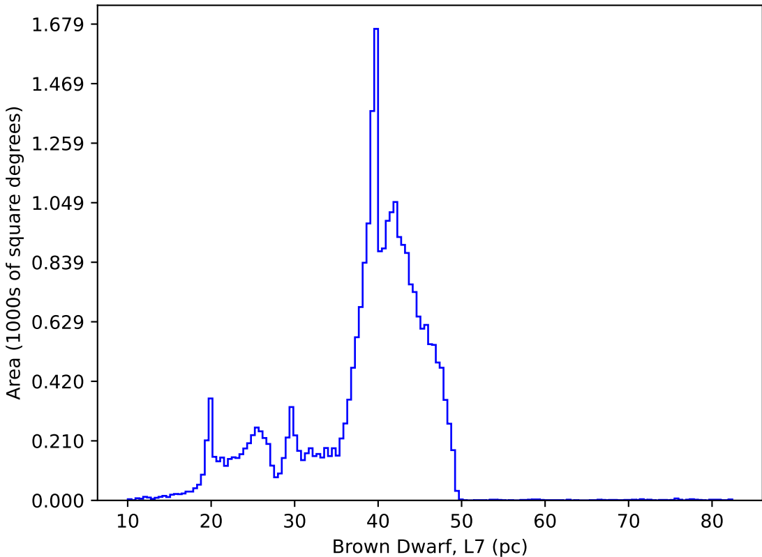
internal_u_expt60_nscale1.5v3.4_10yrs : Brown Dwarf, L7
