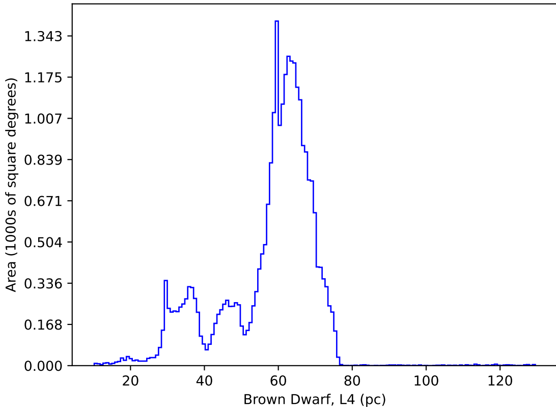
internal_u_expt60_nscale1.5v3.4_10yrs : Brown Dwarf, L4
