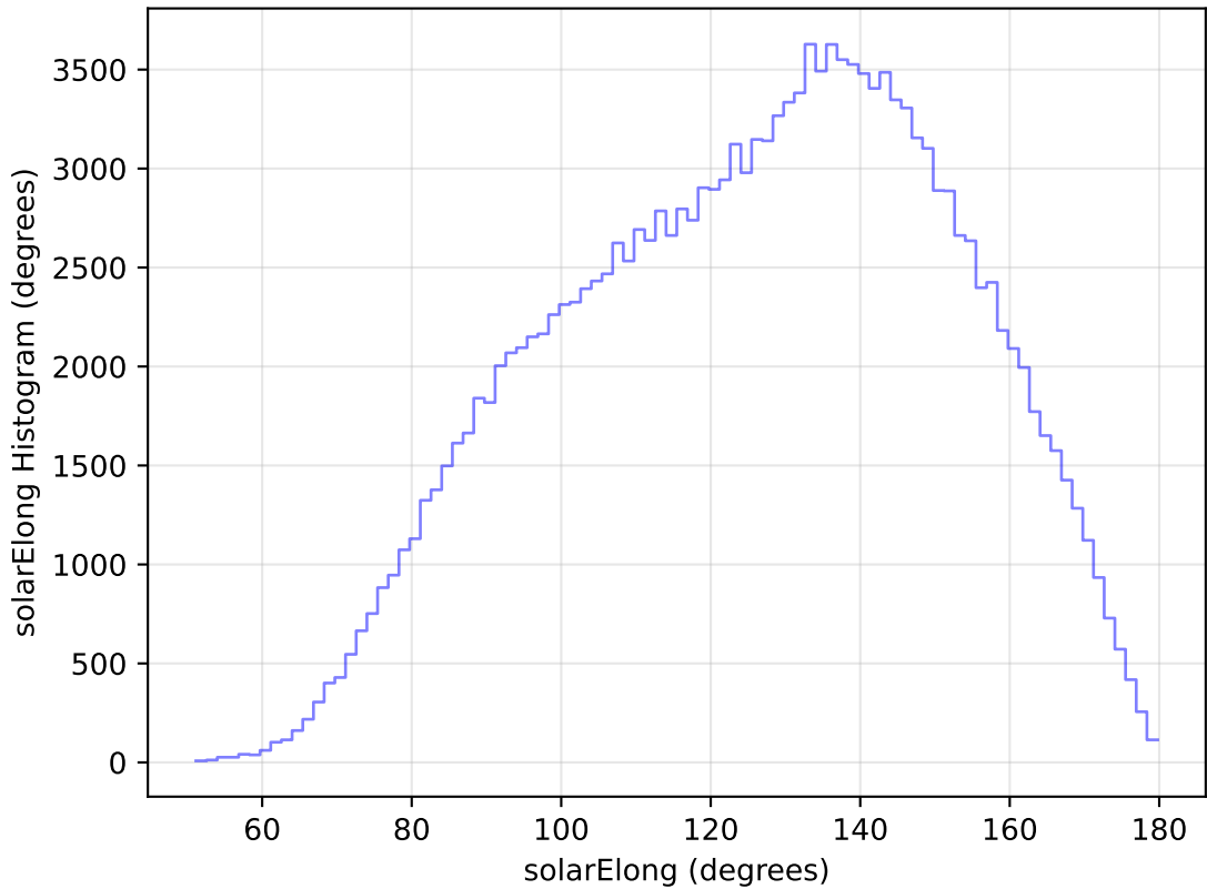
internal_u_expt60_nscale1.5v3.4_10yrs WFD u band: solarElong Histogram
