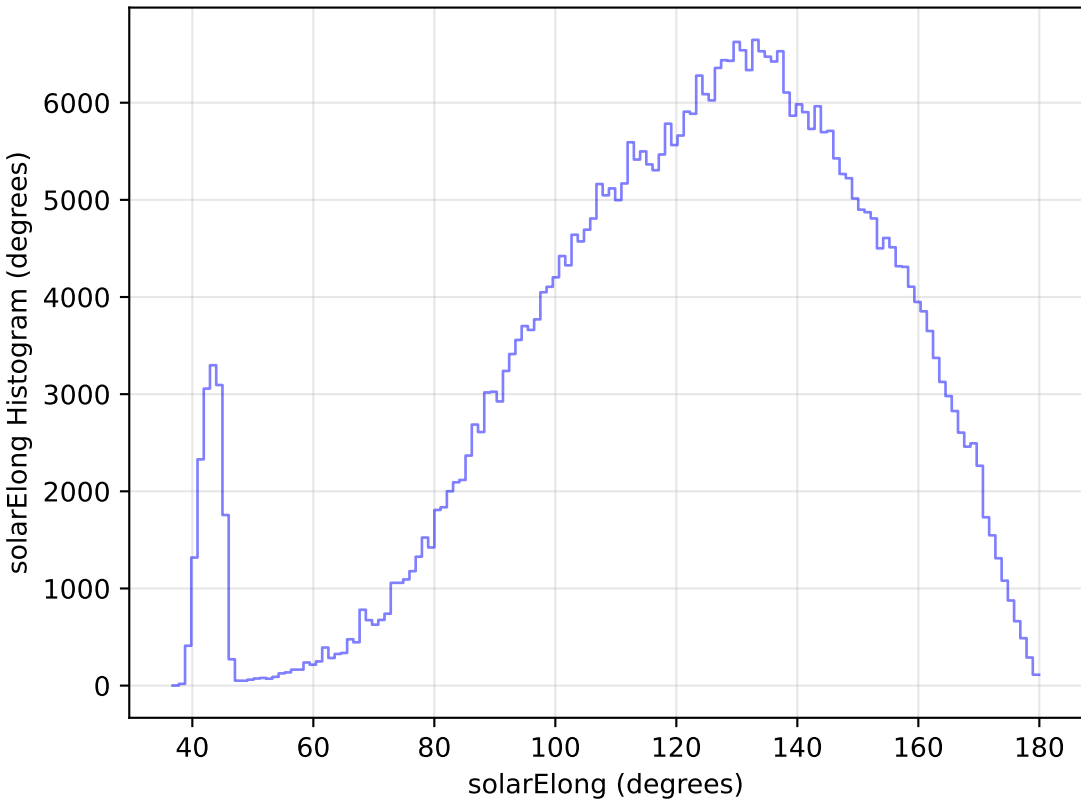
internal_u_expt60_nscale1.5v3.4_10yrs WFD r band: solarElong Histogram
