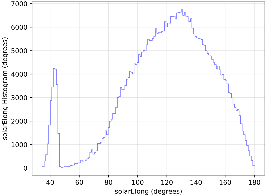
internal_u_expt60_nscale1.5v3.4_10yrs WFD i band: solarElong Histogram
