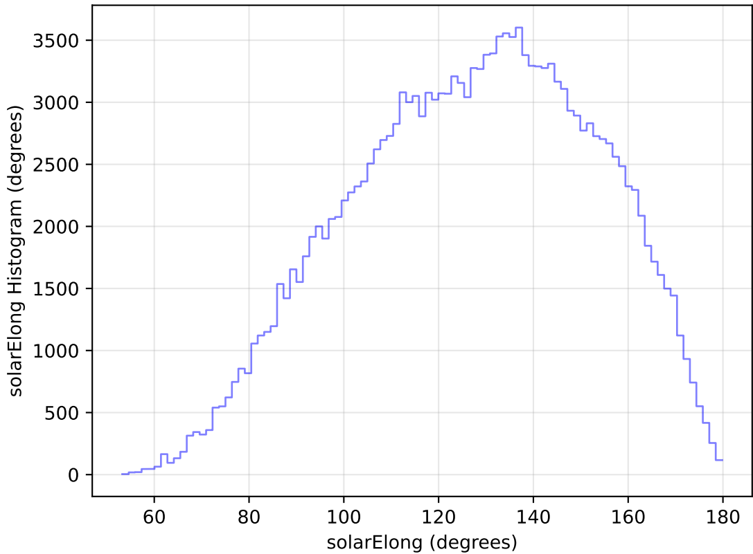
internal_u_expt60_nscale1.5v3.4_10yrs WFD g band: solarElong Histogram
