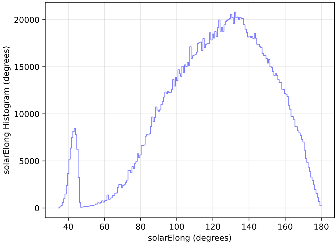
internal_u_expt60_nscale1.5v3.4_10yrs WFD all bands: solarElong Histogram
