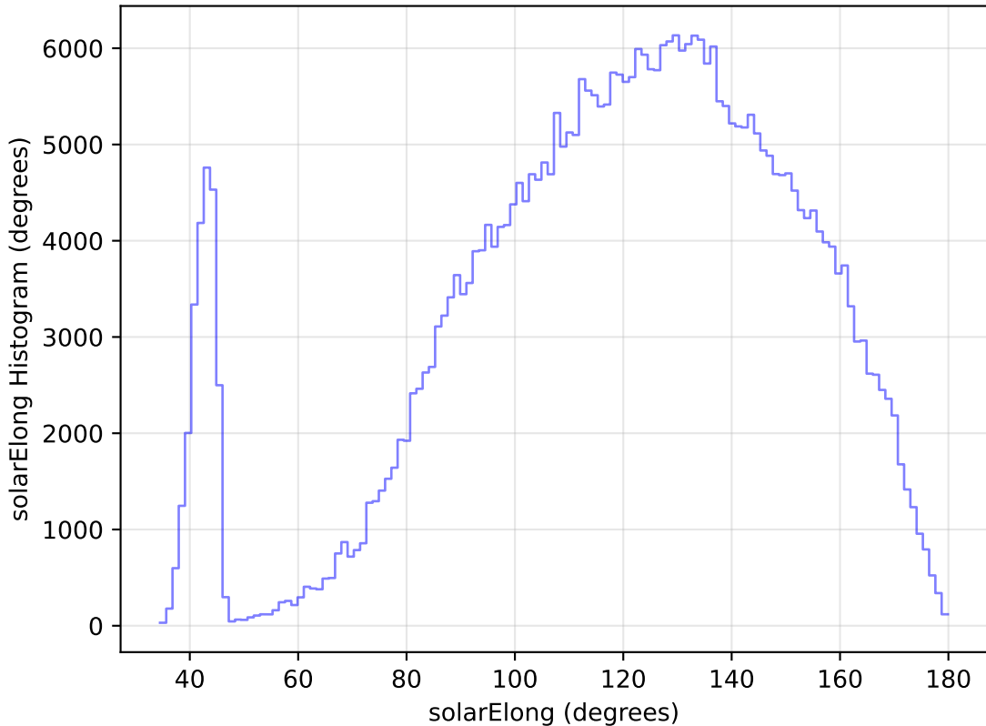
internal_u_expt60_nscale1.5v3.4_10yrs All sky z band: solarElong Histogram
