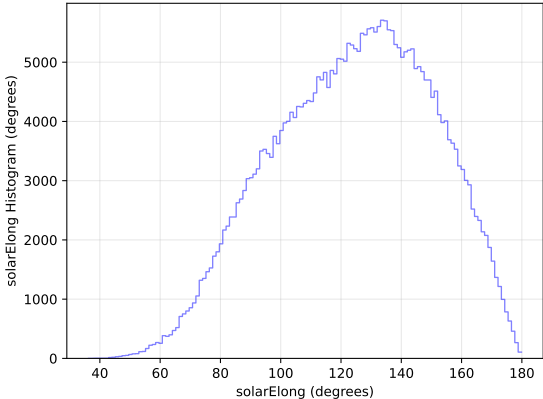
internal_u_expt60_nscale1.5v3.4_10yrs All sky y band: solarElong Histogram
