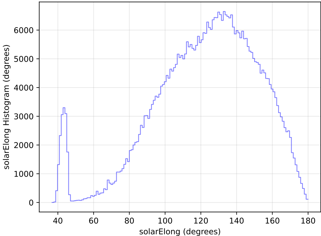
internal_u_expt60_nscale1.5v3.4_10yrs All sky r band: solarElong Histogram
