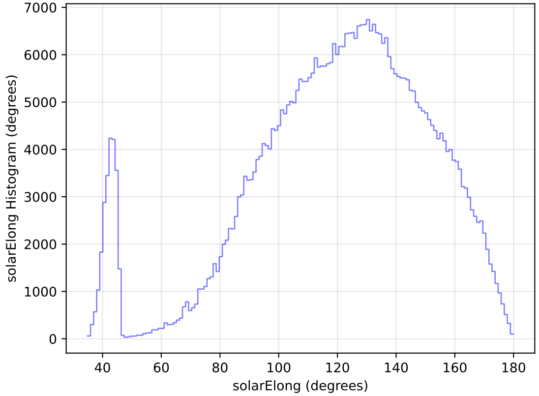
internal_u_expt60_nscale1.5v3.4_10yrs All sky i band: solarElong Histogram
