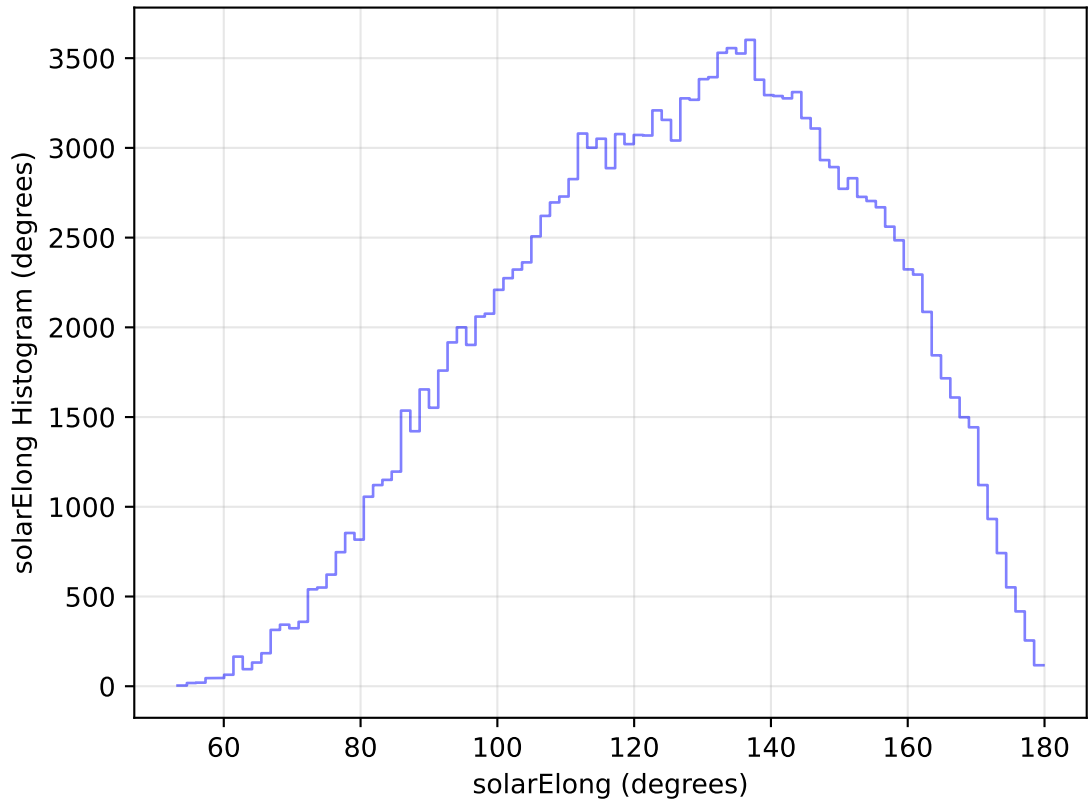
internal_u_expt60_nscale1.5v3.4_10yrs All sky g band: solarElong Histogram
