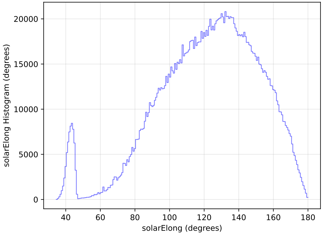
internal_u_expt60_nscale1.5v3.4_10yrs All sky all bands: solarElong Histogram
