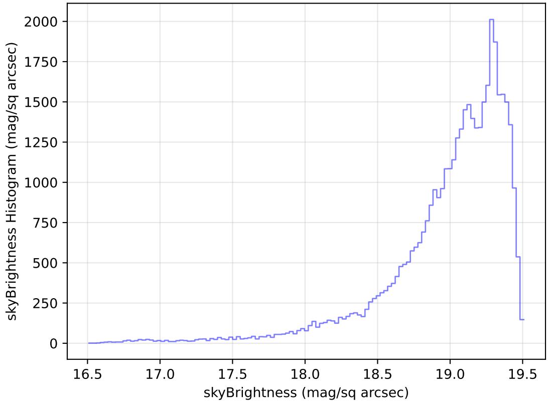
internal_u_expt60_nscale1.5v3.4_10yrs Yr 1 z band: skyBrightness Histogram
