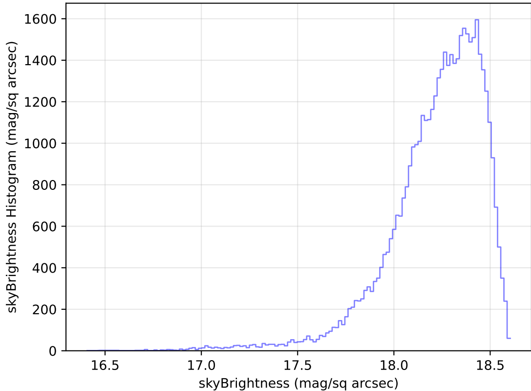
internal_u_expt60_nscale1.5v3.4_10yrs Yr 1 y band: skyBrightness Histogram
