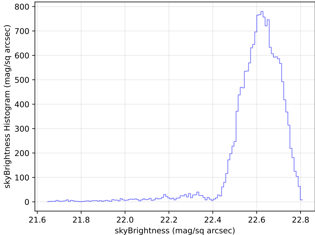
internal_u_expt60_nscale1.5v3.4_10yrs Yr 1 u band: skyBrightness Histogram
