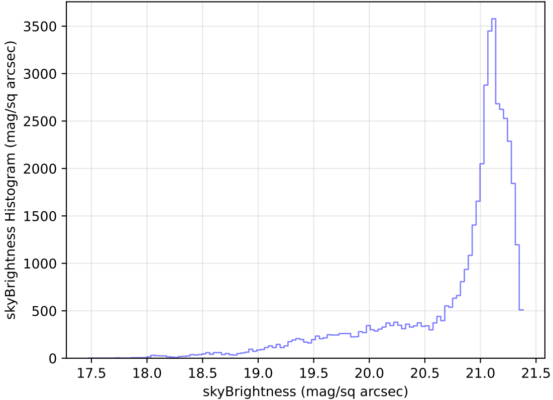
internal_u_expt60_nscale1.5v3.4_10yrs Yr 1 r band: skyBrightness Histogram
