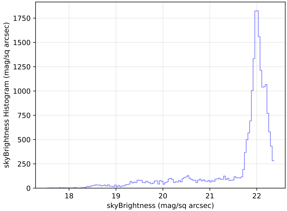
internal_u_expt60_nscale1.5v3.4_10yrs Yr 1 g band: skyBrightness Histogram
