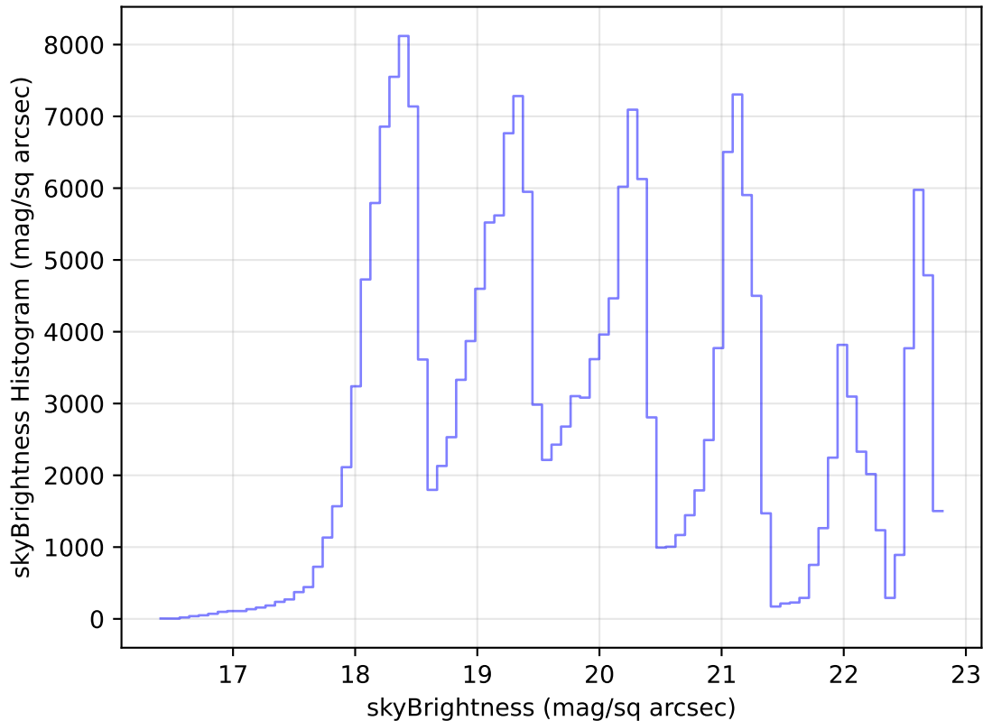
internal_u_expt60_nscale1.5v3.4_10yrs Yr 1 all bands: skyBrightness Histogram
