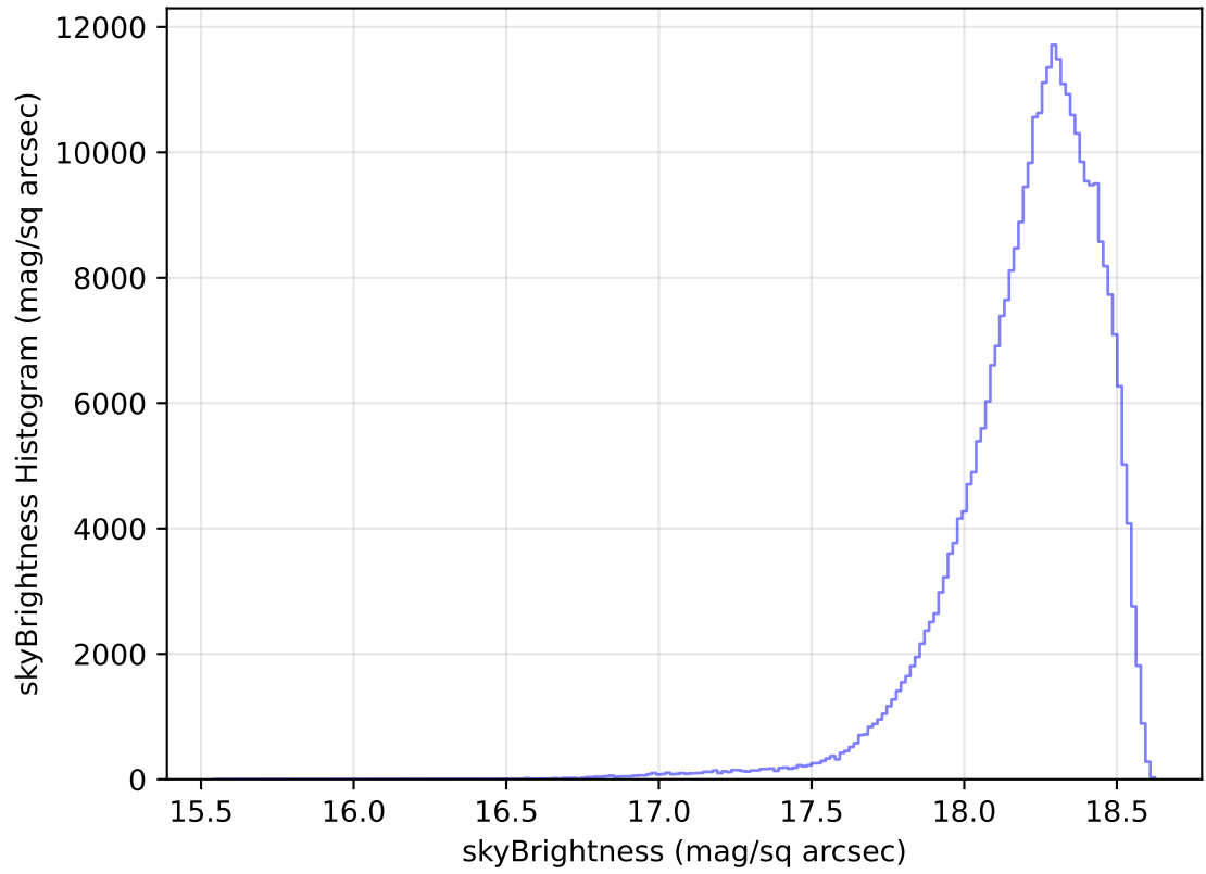
internal_u_expt60_nscale1.5v3.4_10yrs WFD y band: skyBrightness Histogram
