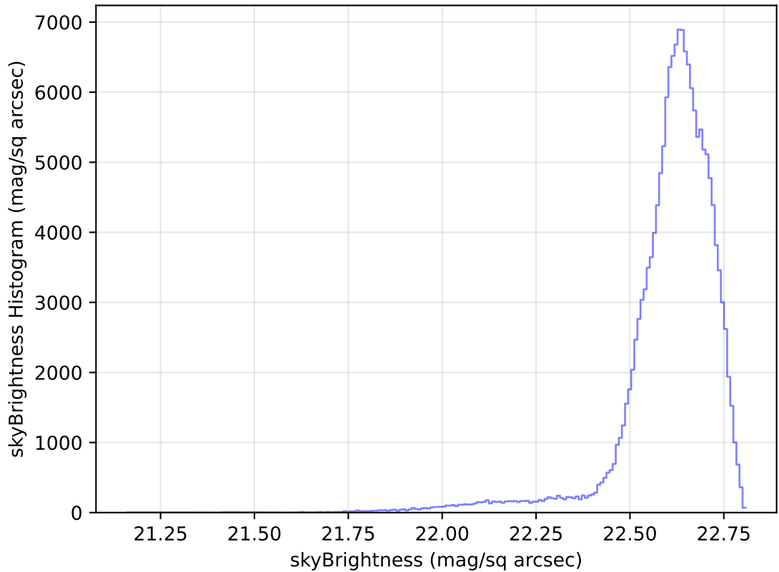
internal_u_expt60_nscale1.5v3.4_10yrs WFD u band: skyBrightness Histogram
