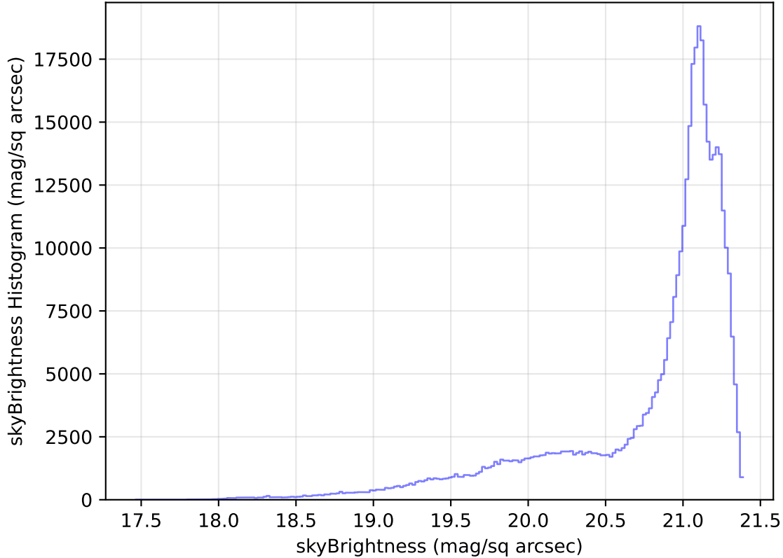
internal_u_expt60_nscale1.5v3.4_10yrs WFD r band: skyBrightness Histogram
