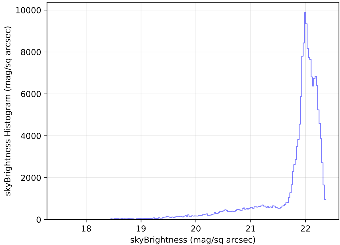
internal_u_expt60_nscale1.5v3.4_10yrs WFD g band: skyBrightness Histogram
