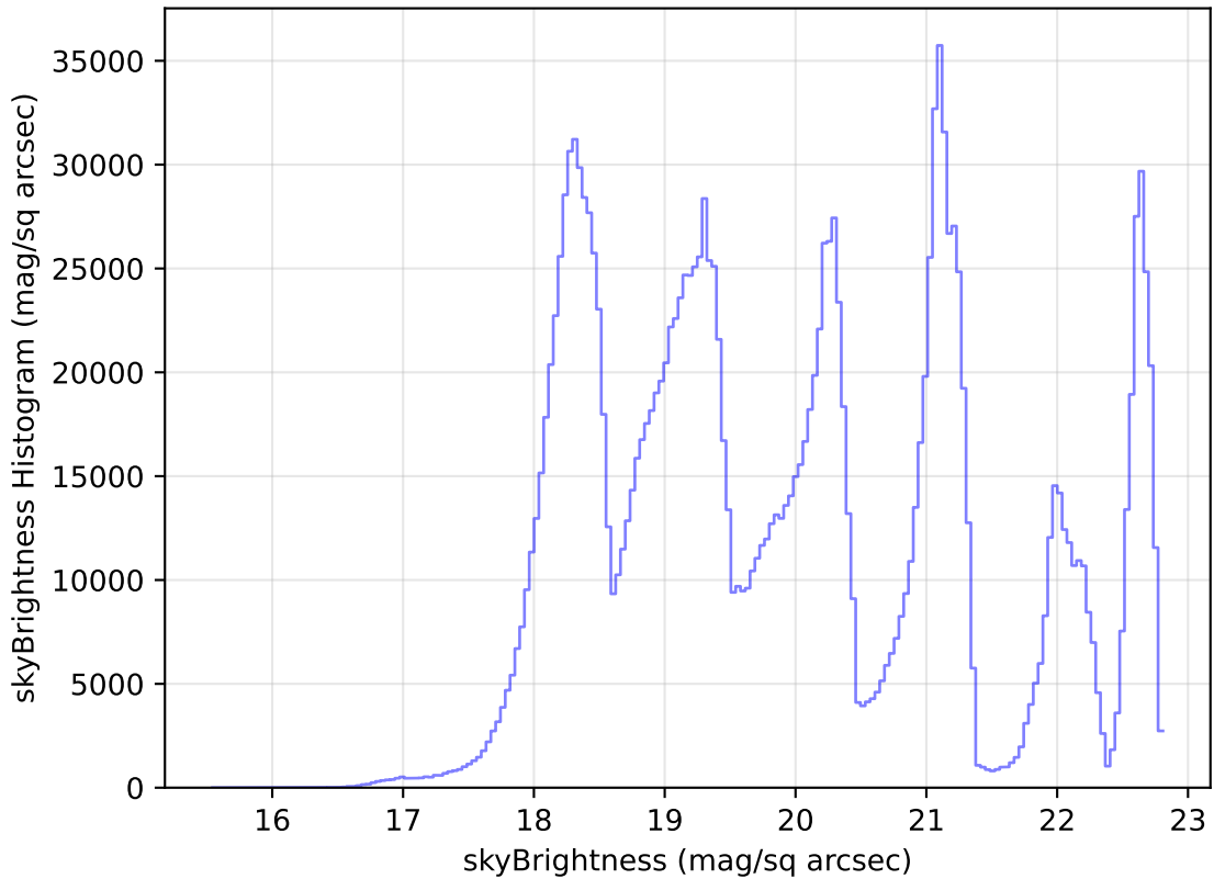
internal_u_expt60_nscale1.5v3.4_10yrs WFD all bands: skyBrightness Histogram
