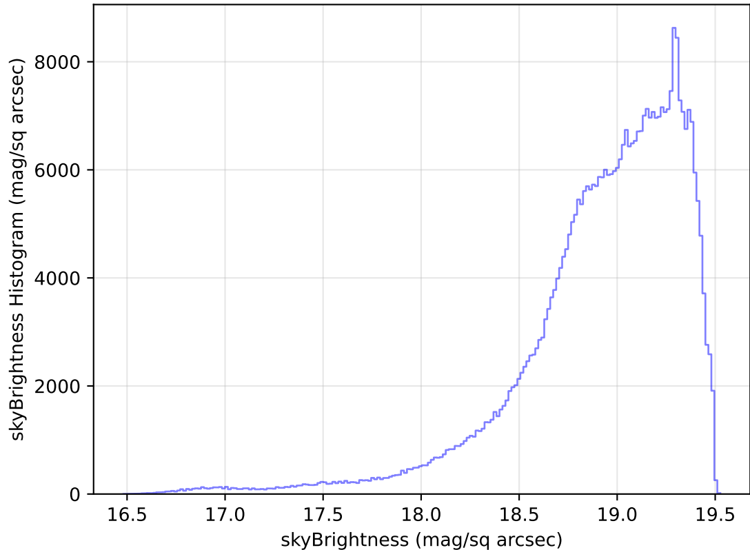
internal_u_expt60_nscale1.5v3.4_10yrs All sky z band: skyBrightness Histogram
