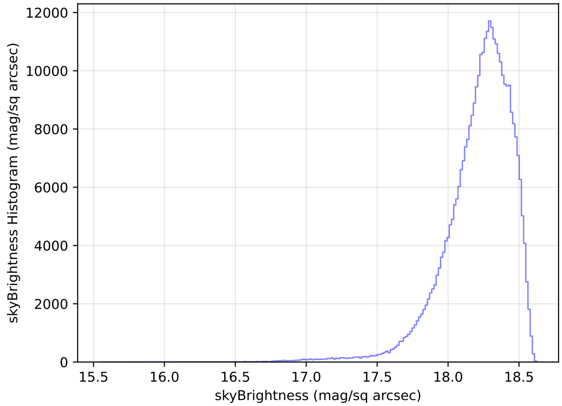
internal_u_expt60_nscale1.5v3.4_10yrs All sky y band: skyBrightness Histogram
