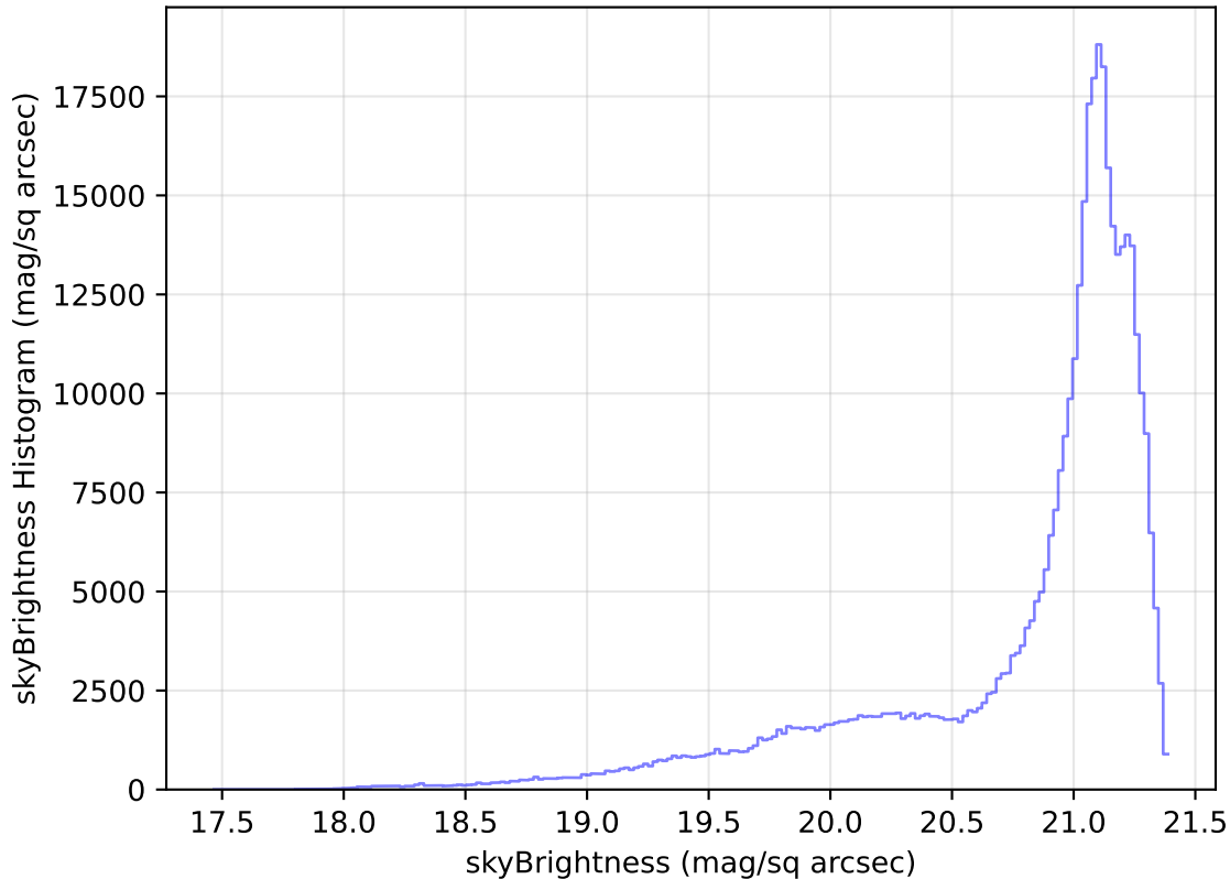
internal_u_expt60_nscale1.5v3.4_10yrs All sky r band: skyBrightness Histogram
