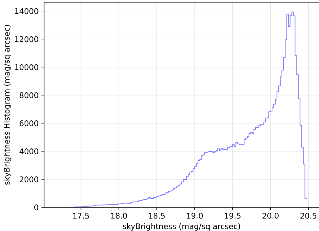
internal_u_expt60_nscale1.5v3.4_10yrs All sky i band: skyBrightness Histogram
