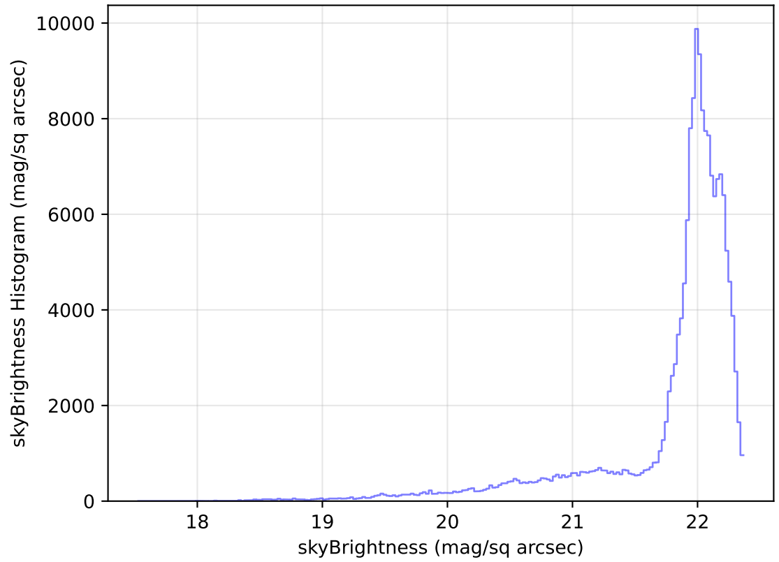
internal_u_expt60_nscale1.5v3.4_10yrs All sky g band: skyBrightness Histogram
