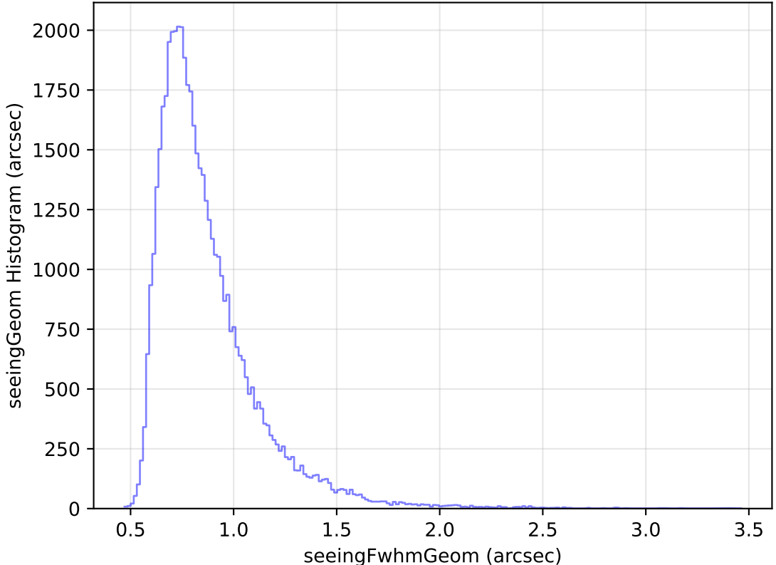
internal_u_expt60_nscale1.5v3.4_10yrs Yr 1 i band: seeingGeom Histogram
